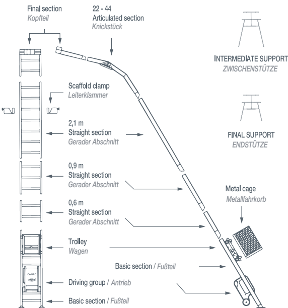
VERTICAL ASSEMBLY / VERTIKALE MONTAGE
